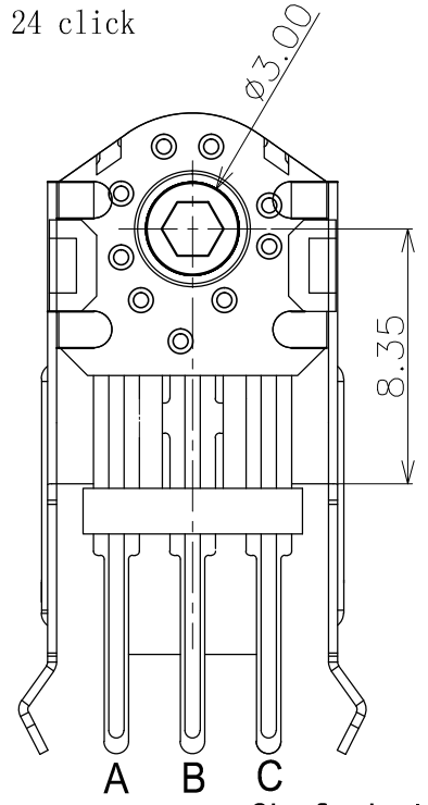
Shaft hole shape and dimension
