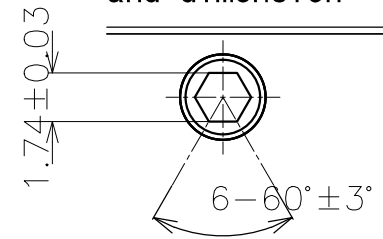
Shaft hole shape and dimension
