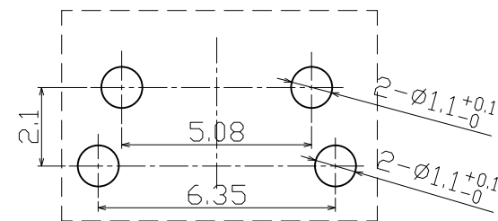
P.C.B mounting hole detail
